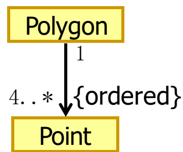
(b)单向关联
